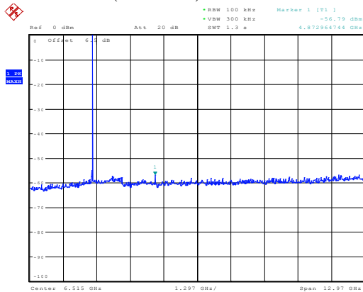
Middle Channel(2 441 MHz): 30 MHz ~ 13 GHz
