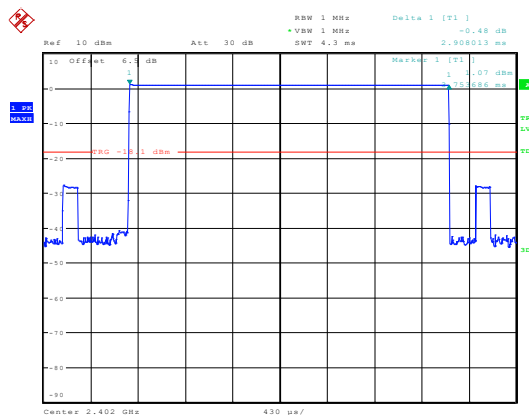
Figure 5. Plot of the Time of Occupancy (Conducted)
