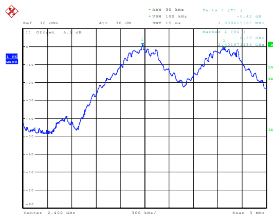
Figure 2. Plot of the Carrier Frequency Separation (Conducted)
