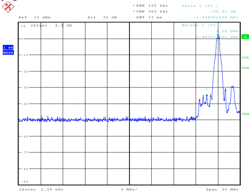
Figure 6. Plot of the Band Edge (Conducted)
