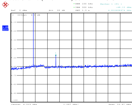
Figure 8. Plot of the Spurious RF conducted emissions - GFSK
