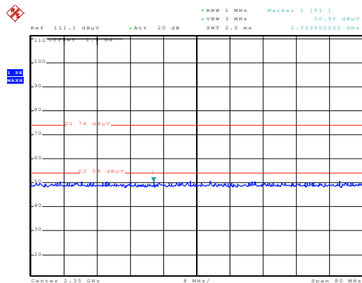
Figure 7. Plot of the Band Edge (Radiated) - GFSK
