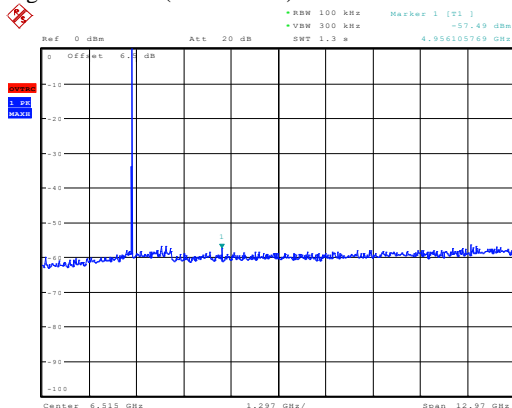
Highest Channel(2 480 MHz): 30 MHz ~ 13 GHz
