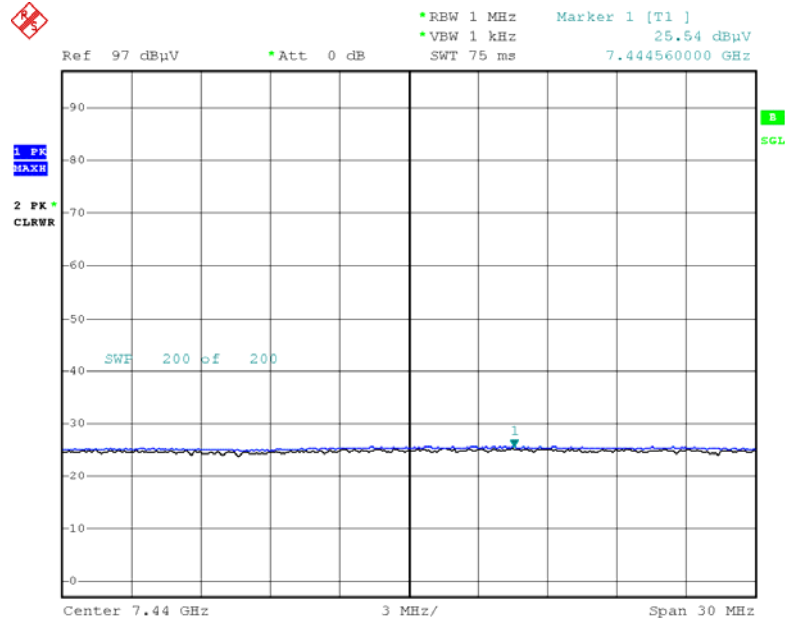
Radiated Spurious Emissions plot – Average Reading (8DPSK, Ch.78 3rd Harmonic)
