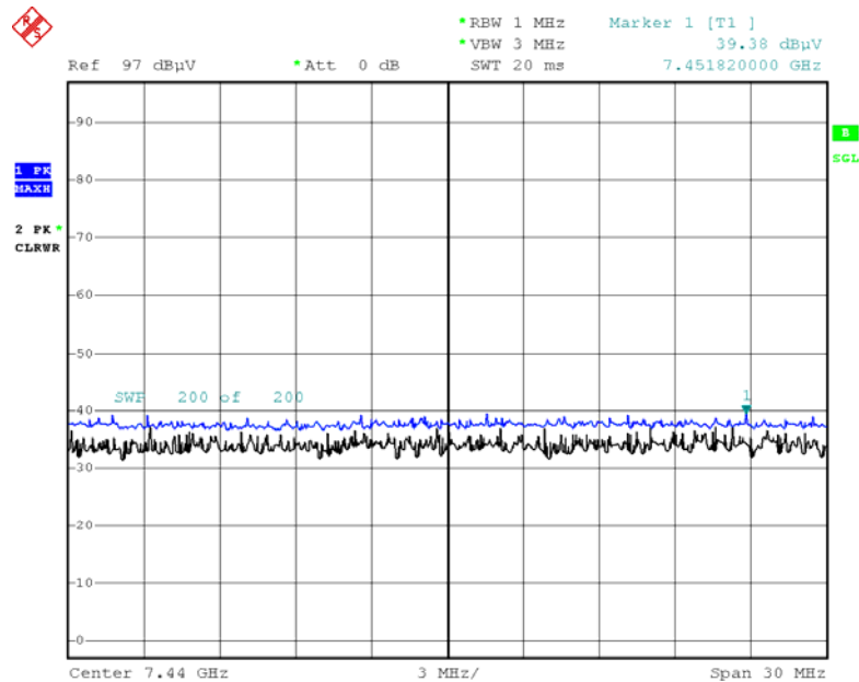
Radiated Spurious Emissions plot – Peak Reading (8DPSK, Ch.78 3rd Harmonic)
