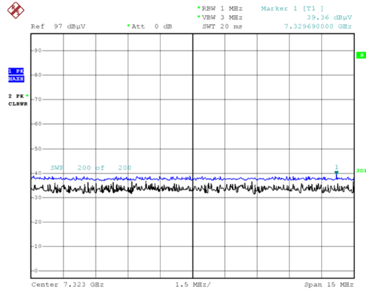
Radiated Spurious Emissions plot – Peak Reading (8DPSK, Ch.39 3rd Harmonic, X-H)
