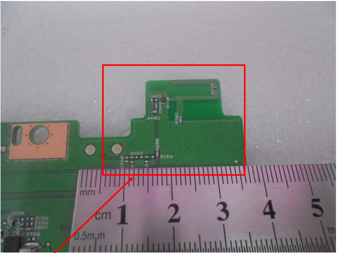
BT Antenna
