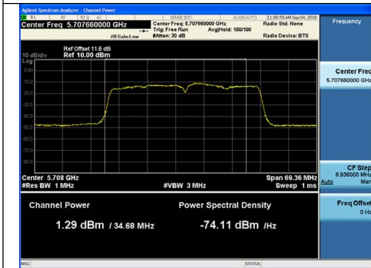
802.11ac_VHT40 UNII 2C Band Average Power CH.142
