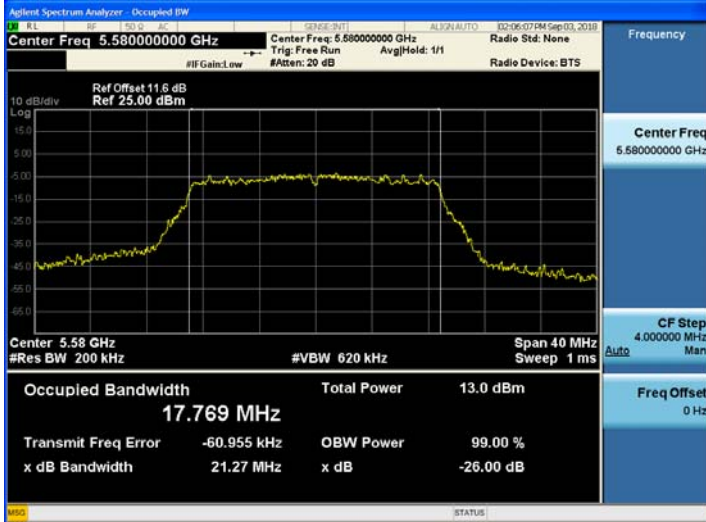
802.11ac_VHT20 UNII 2C BAND 26dB Bandwidth(CH 116)
