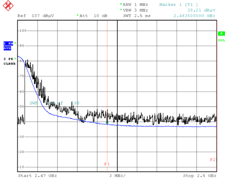
Radiated Restricted Band Edges plot – Average Reading (802.11n(HT20) Ch.11)
