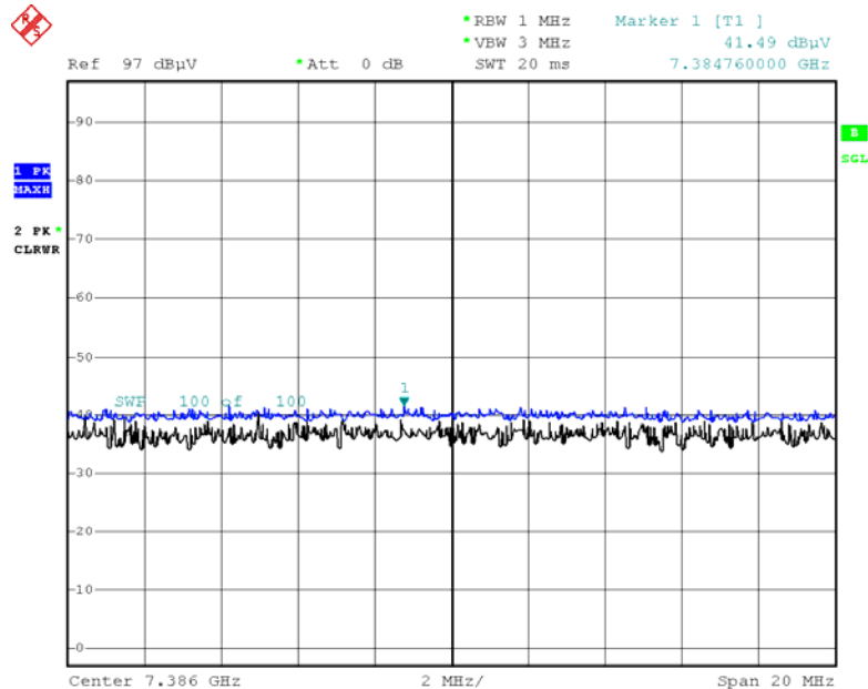
Radiated Spurious Emissions plot – Peak Reading (802.11g, Ch.11 3rd Harmonic, X-H)
