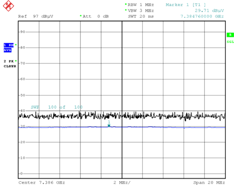
Radiated Spurious Emissions plot – Average Reading (802.11g, Ch.11 3rd Harmonic, X-H)
