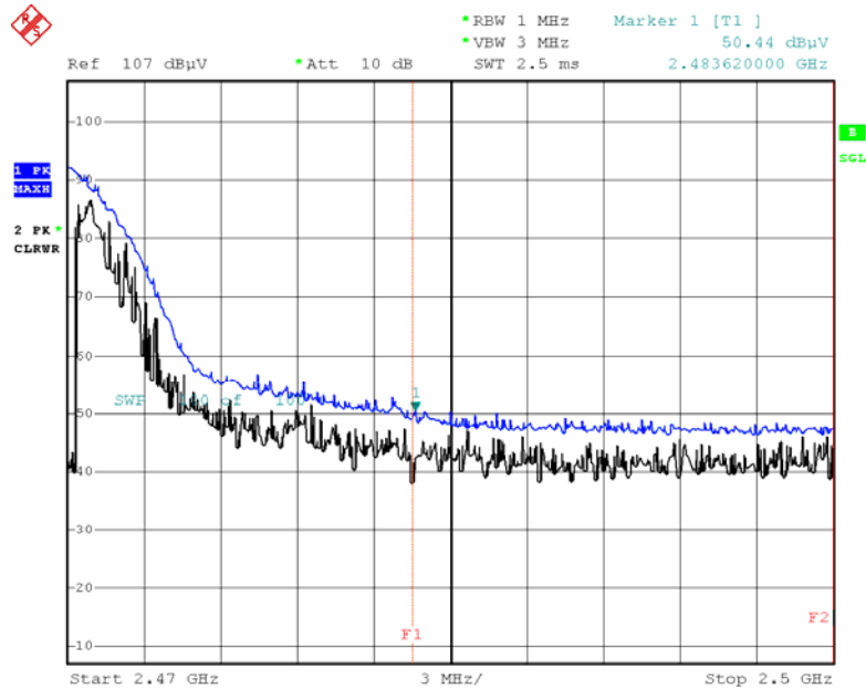
Radiated Restricted Band Edges plot – Peak Reading (802.11n(HT20) Ch.11)
