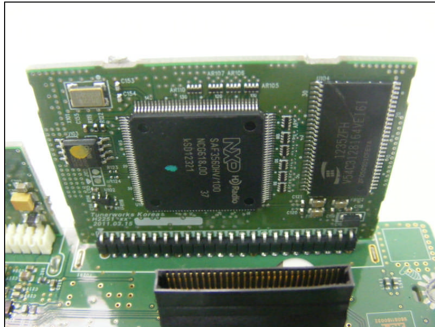
Bottom view of Audio PCB
