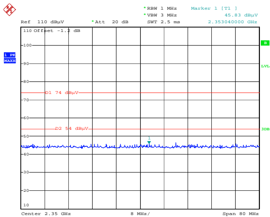
Figure 7. Plot of the Band Edge (Radiated) - GFSK
