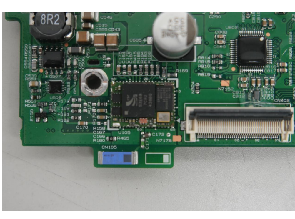
View of bluetooth module after taking off
