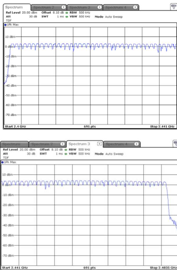
Figure 4. Plot of the Number of Hopping Channels (Conducted)
