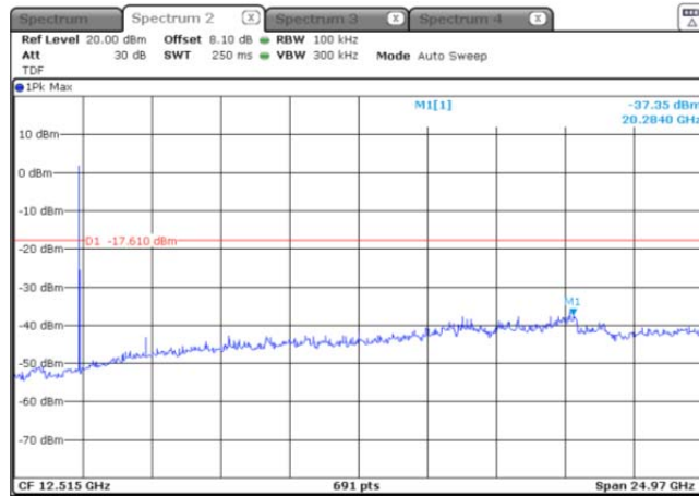
Figure 8. Plot of the Spurious RF conducted emissions
