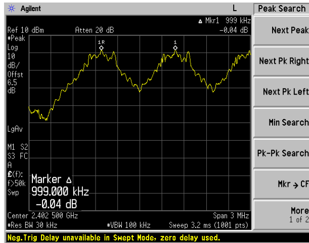
Figure 2. Plot of the Carrier Frequency Separation (Conducted)
