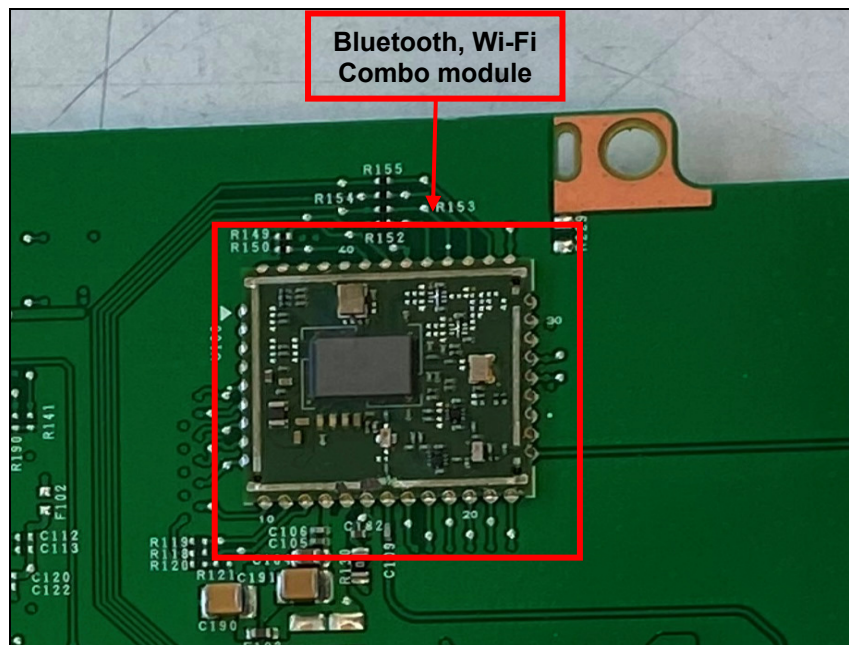
View of Bluetooth, Wi-Fi Combo module
