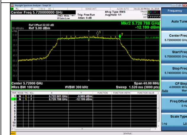
802.11ac_VHT20 CH.144
