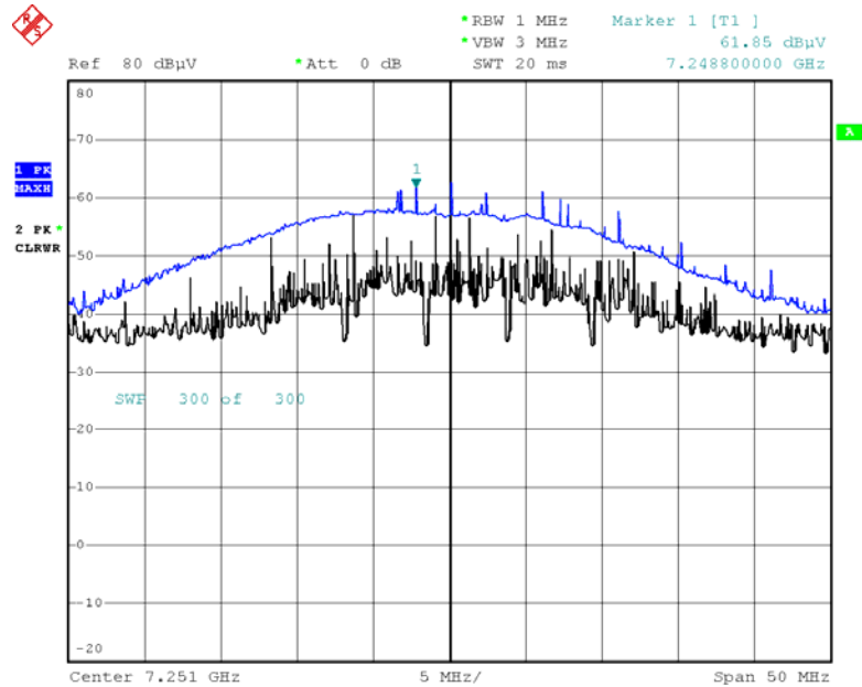
Radiated Spurious Emissions plot – Peak Reading (802.11g, Ch.2 3rd Harmonic)
