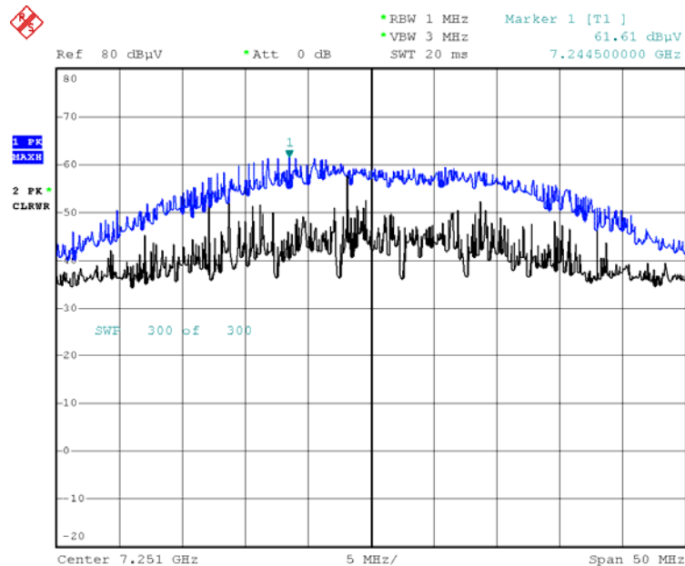
Radiated Spurious Emissions plot – Peak Reading (802.11n(20M), Ch.2 3rd Harmonic)
