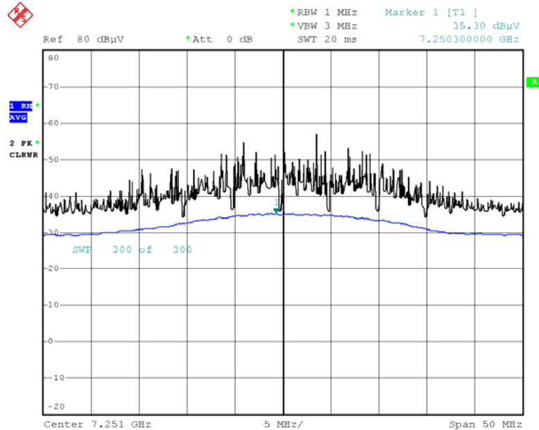
Radiated Spurious Emissions plot – Average Reading (802.11n(20M), Ch.2 3rd Harmonic)
