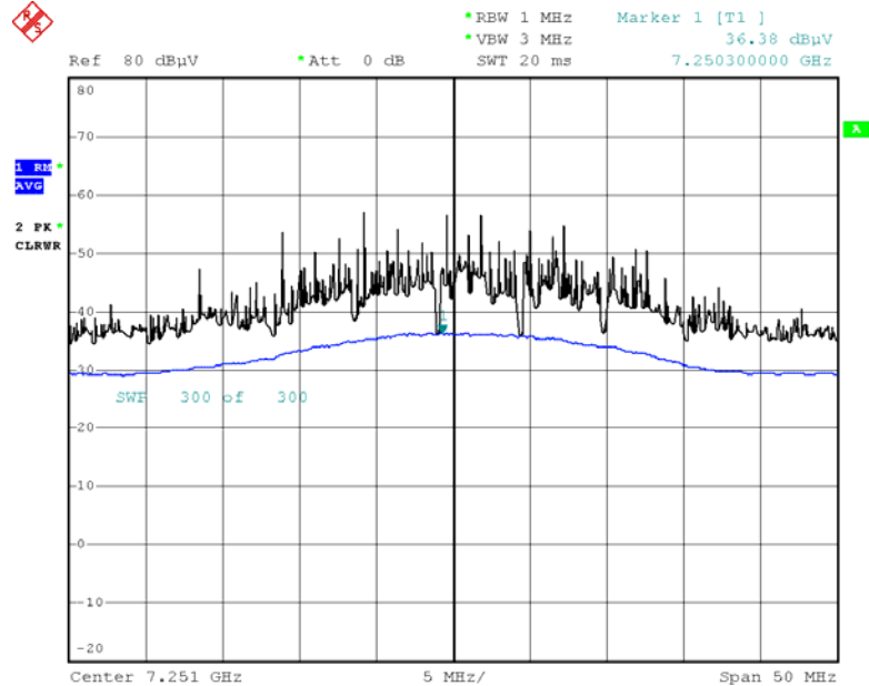
Radiated Spurious Emissions plot – Average Reading (802.11g, Ch.2 3rd Harmonic)
