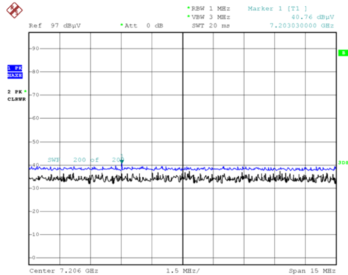
Radiated Spurious Emissions plot – (GFSK, Ch.0 3rd Harmonic, X-V)
