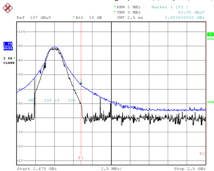
Radiated Restricted Band Edges plot – ( \pi/4 DQPSK, Ch.78, X-V)
