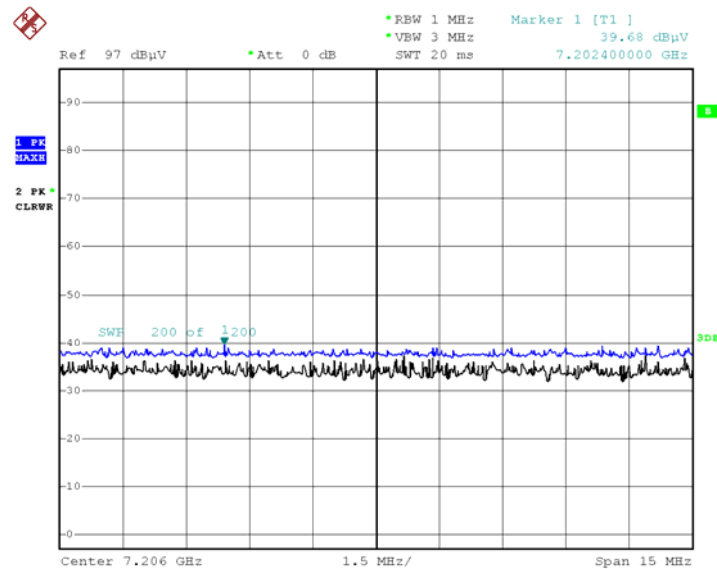
Radiated Spurious Emissions plot – ( \pi/4 DQPSK, Ch.0 3rd Harmonic, X-V)
