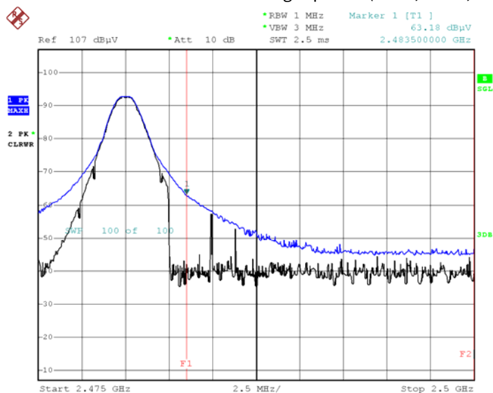
Radiated Restricted Band Edges plot – (GFSK, Ch.78, X-V)
