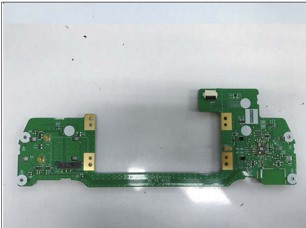
Top view of Sub PCB2 (without Shielding can)
