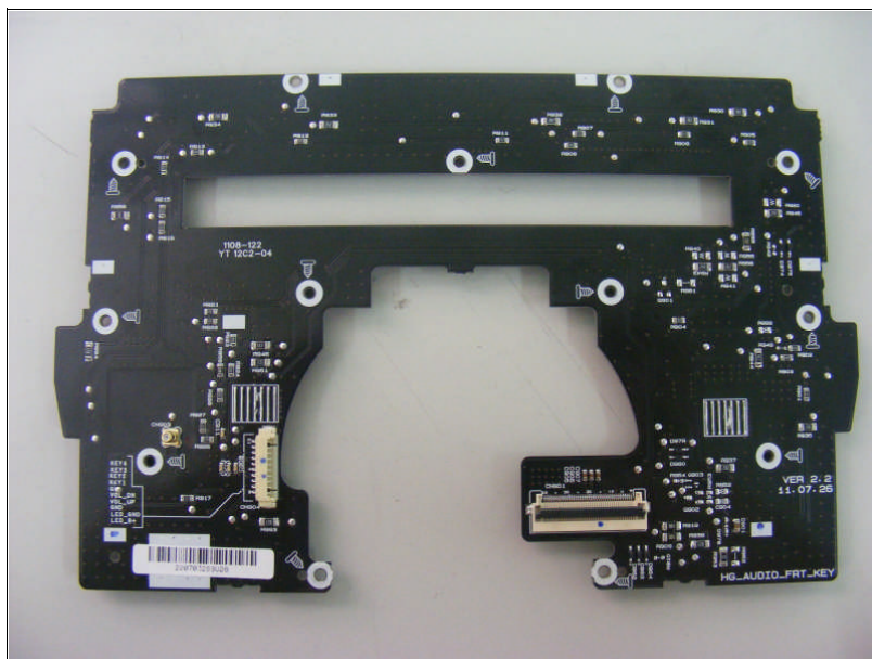
Bottom view of Keypad
