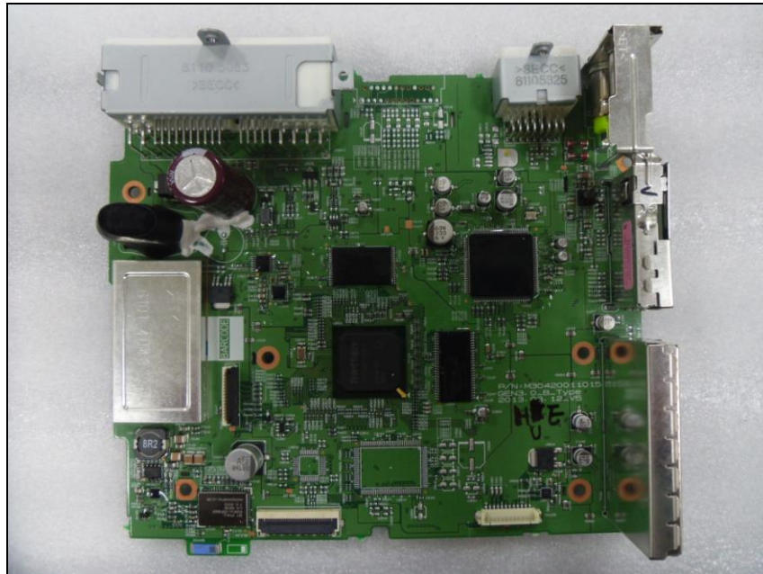
Top view of Main PCB (Without shilding cap)
