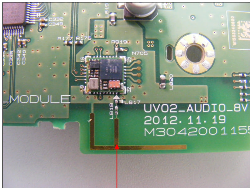
Bluetooth Antenna
