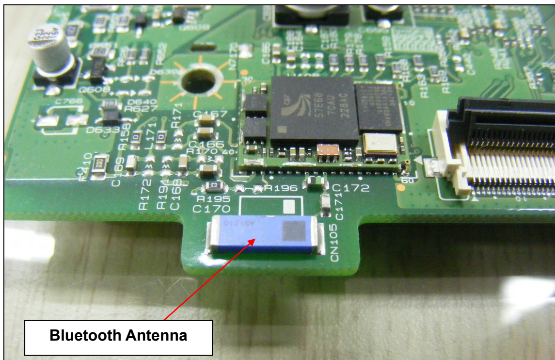
Top view of Bluetooth Antenna
