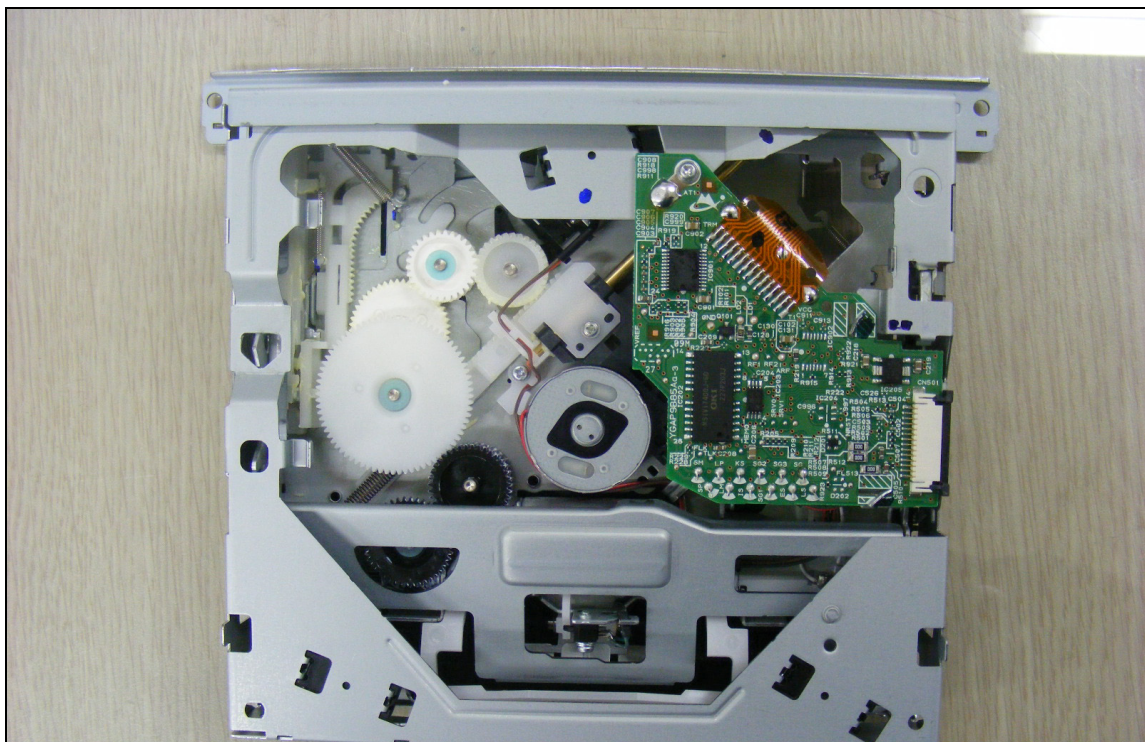
Bottom view of CD Player
