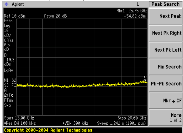
Middle Channel(2 441 MHz): 13 GHz ~ 26 GHz
