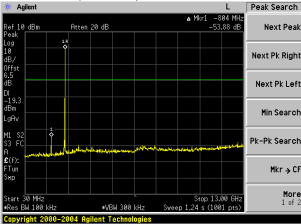
Middle Channel(2 441 MHz): 30 MHz ~ 13 GHz
