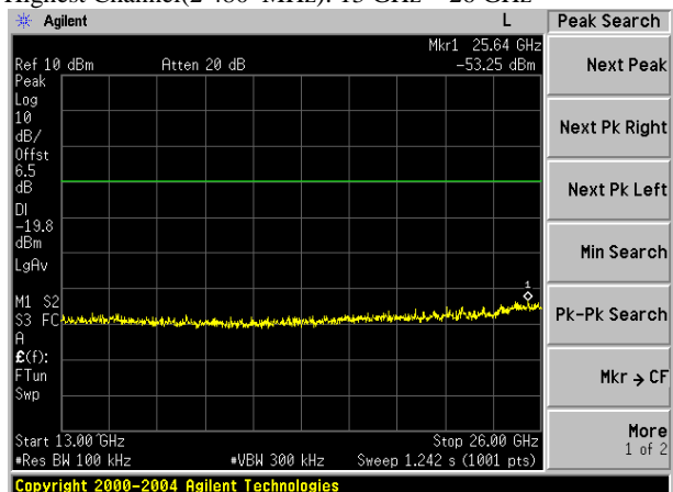
Highest Channel(2 480 MHz): 13 GHz ~ 26 GHz
