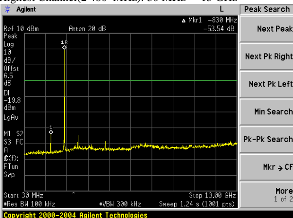
Highest Channel(2 480 MHz): 30 MHz ~ 13 GHz
