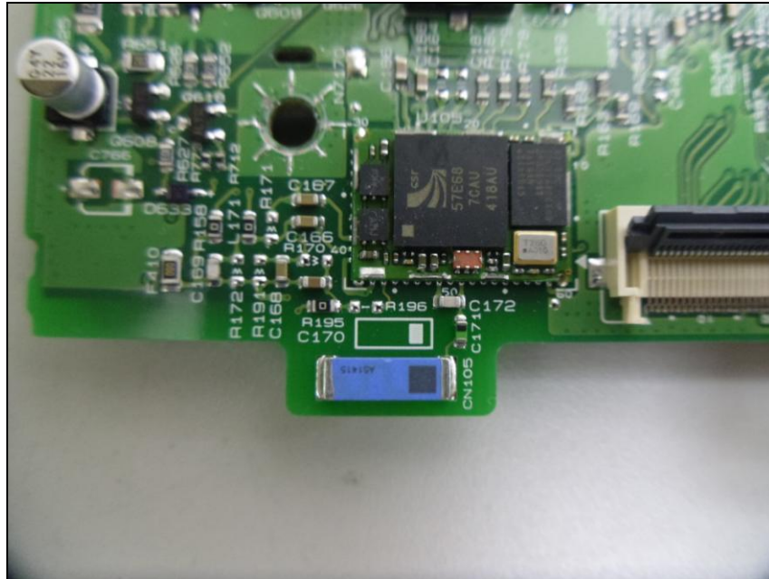
Top view of Module and Chip Antenna
