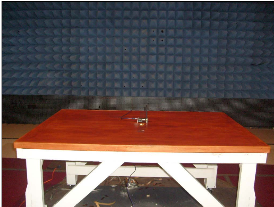
Photograph 2. Omni Antenna
