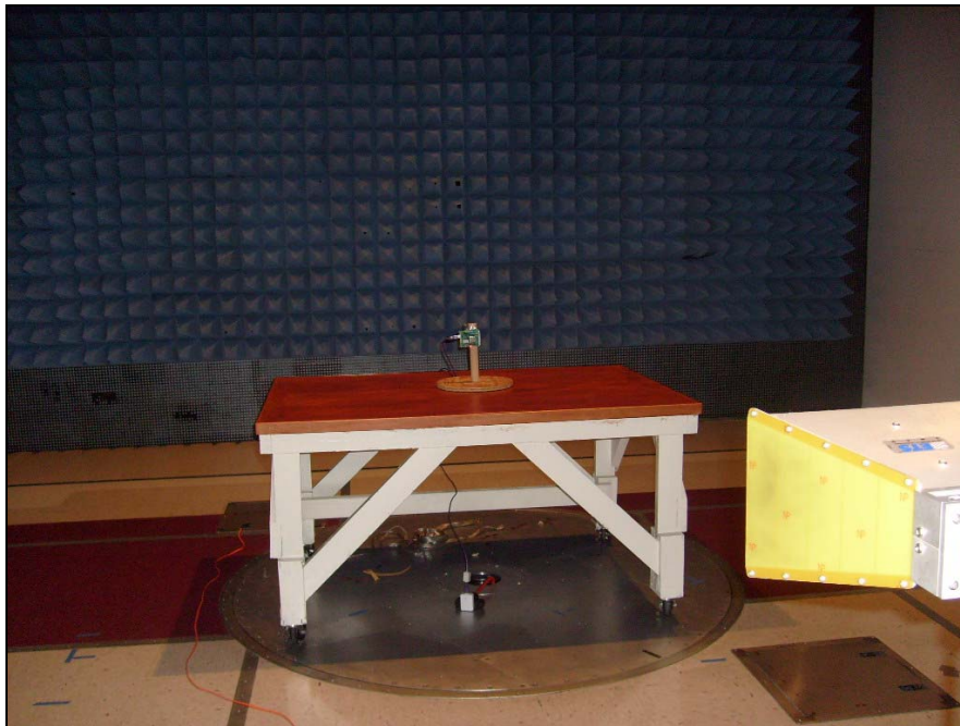
Photograph 4. PCB Horn
