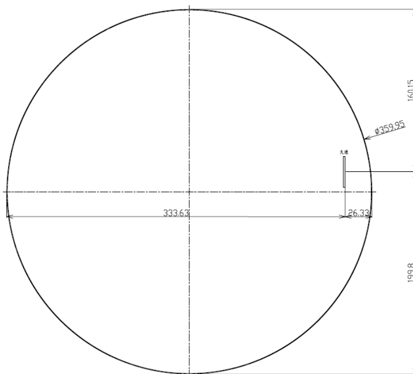
Fig.6 Antenna position of EUT (Front view)
