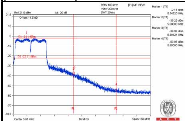
802.11ac (VHT40) MODULATION (CH 110: 5550MHz)
