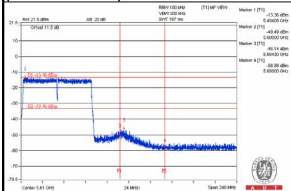
802.11ac (VHT80) MODULATION (CH 106: 5530MHz)
