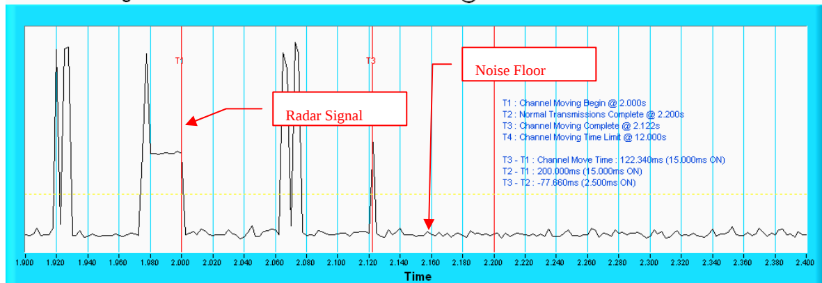
Channel Closing Transmission Time & Channel Move Time @ AC80 -106
