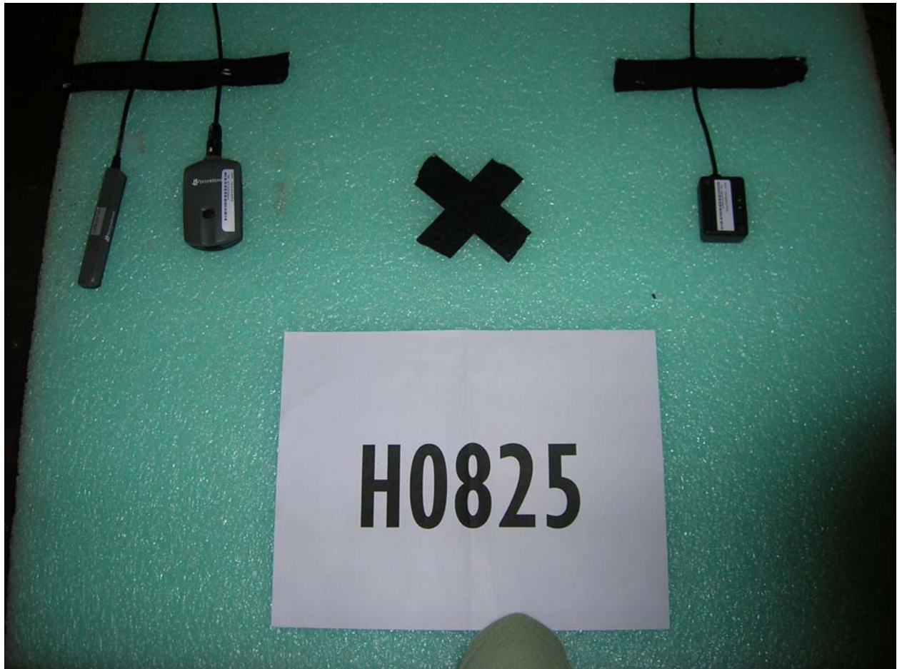
Radiated Emissions Setup Receiver shown with Head Tracker Transmitter for communications.
