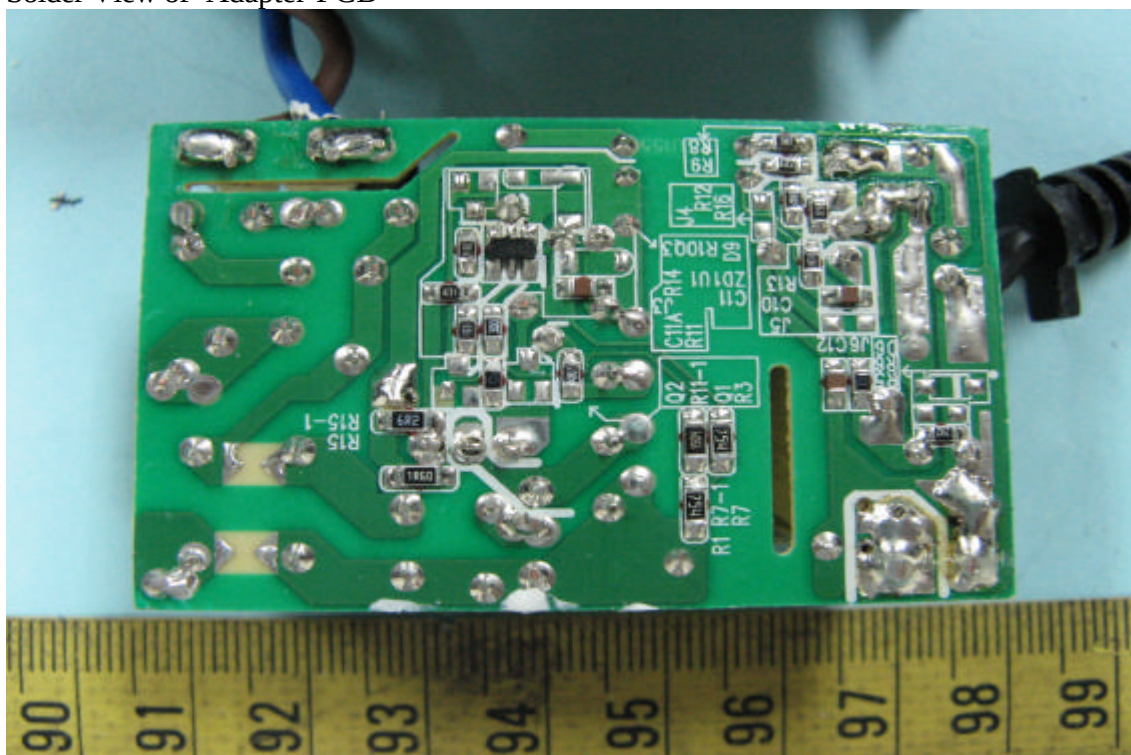
Solder View of Adapter'PCB
