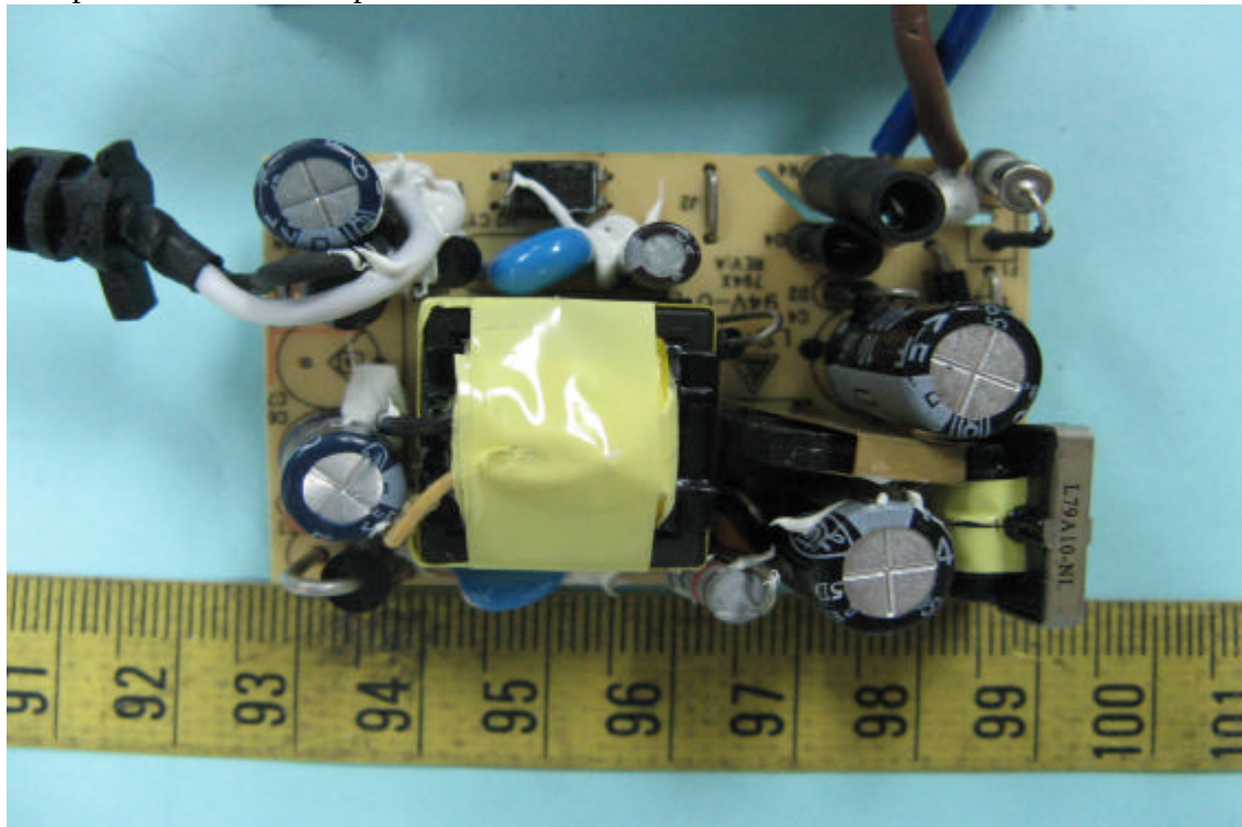
Component View of Adapter'PCB
