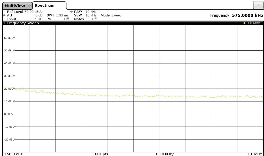
172416_103.png: Spurious emissions from 150 kHz to 1 MHz
