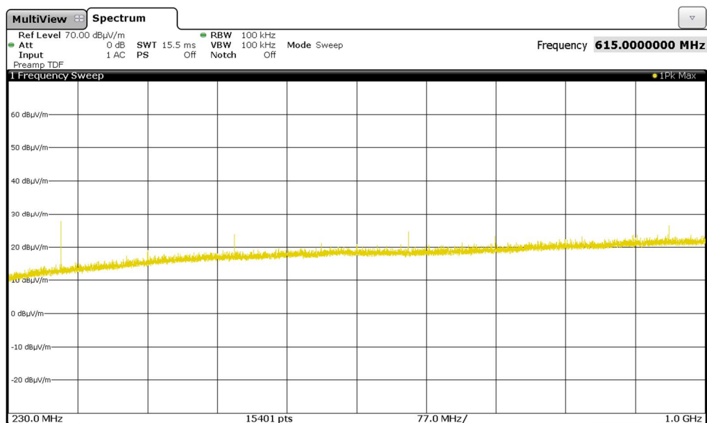
172416_105.png: Spurious emissions from 230 MHz to 1 GHz
