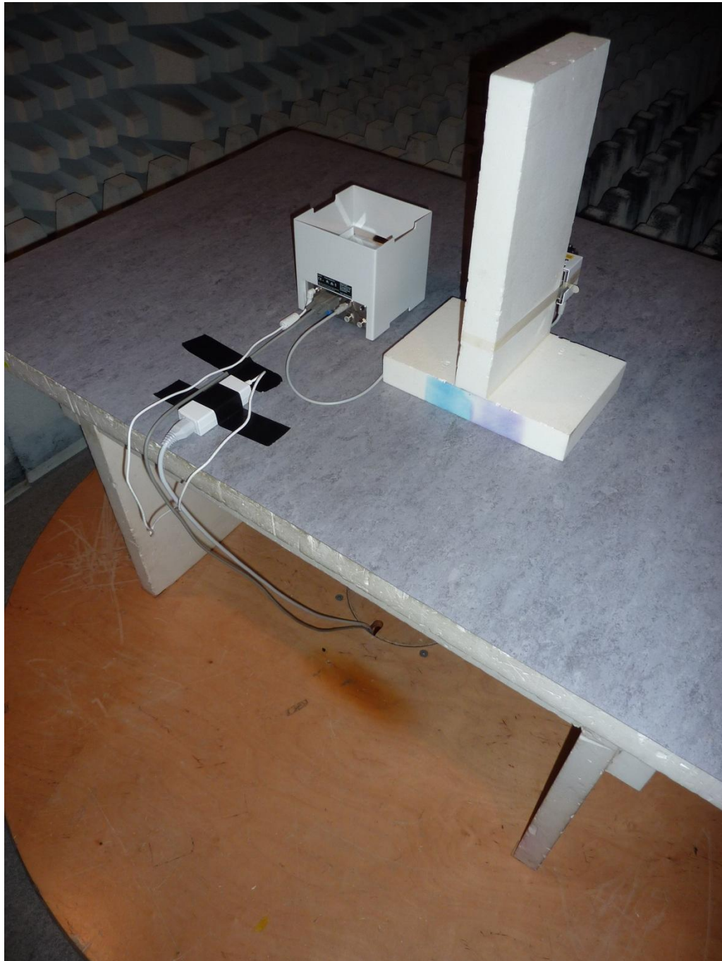
161006_1a.jpg: QLX45 Liquid Dosing Module, test setup fully anechoic chamber
