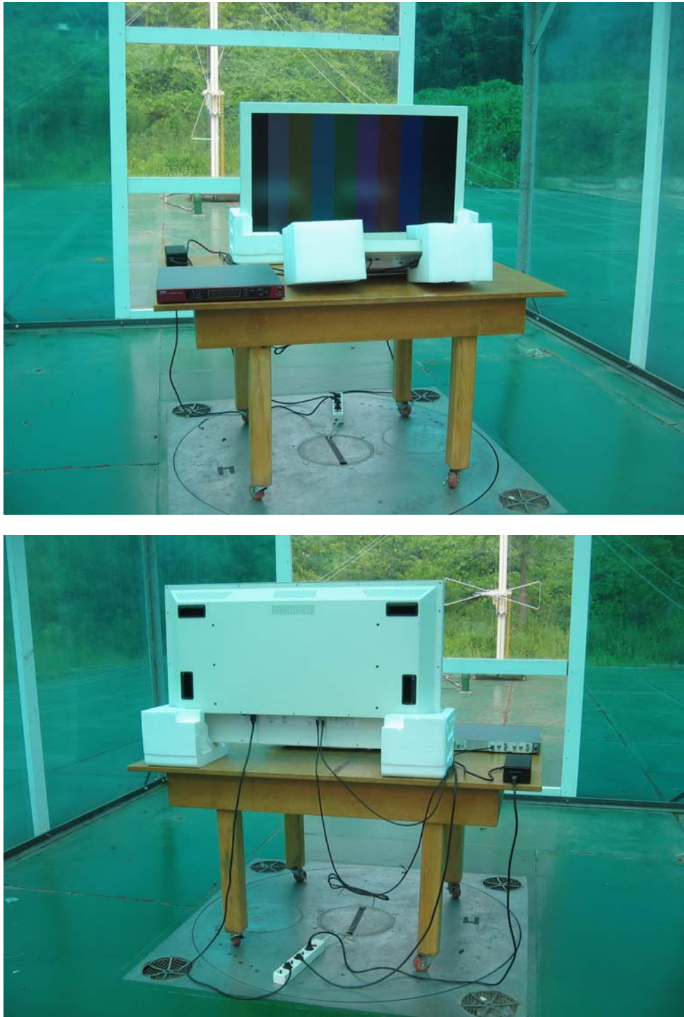
Figure 4 Photo of Radiated emission test setup: SDI Mode
