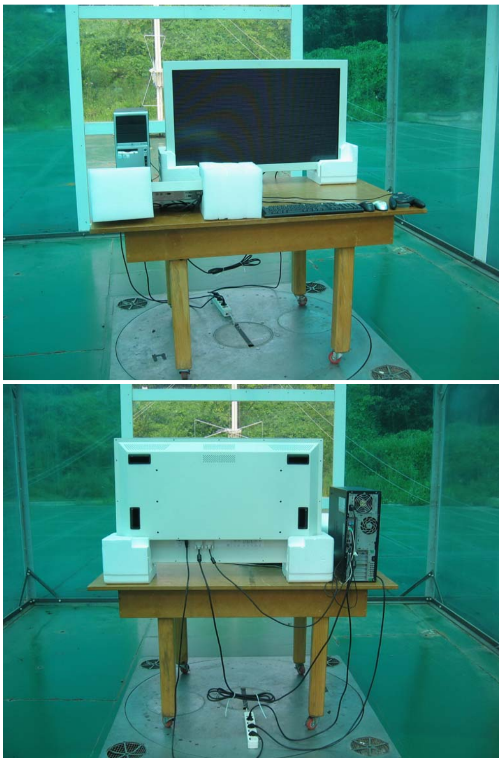
Figure 3 Photo of Radiated emission test setup: DVI Mode
