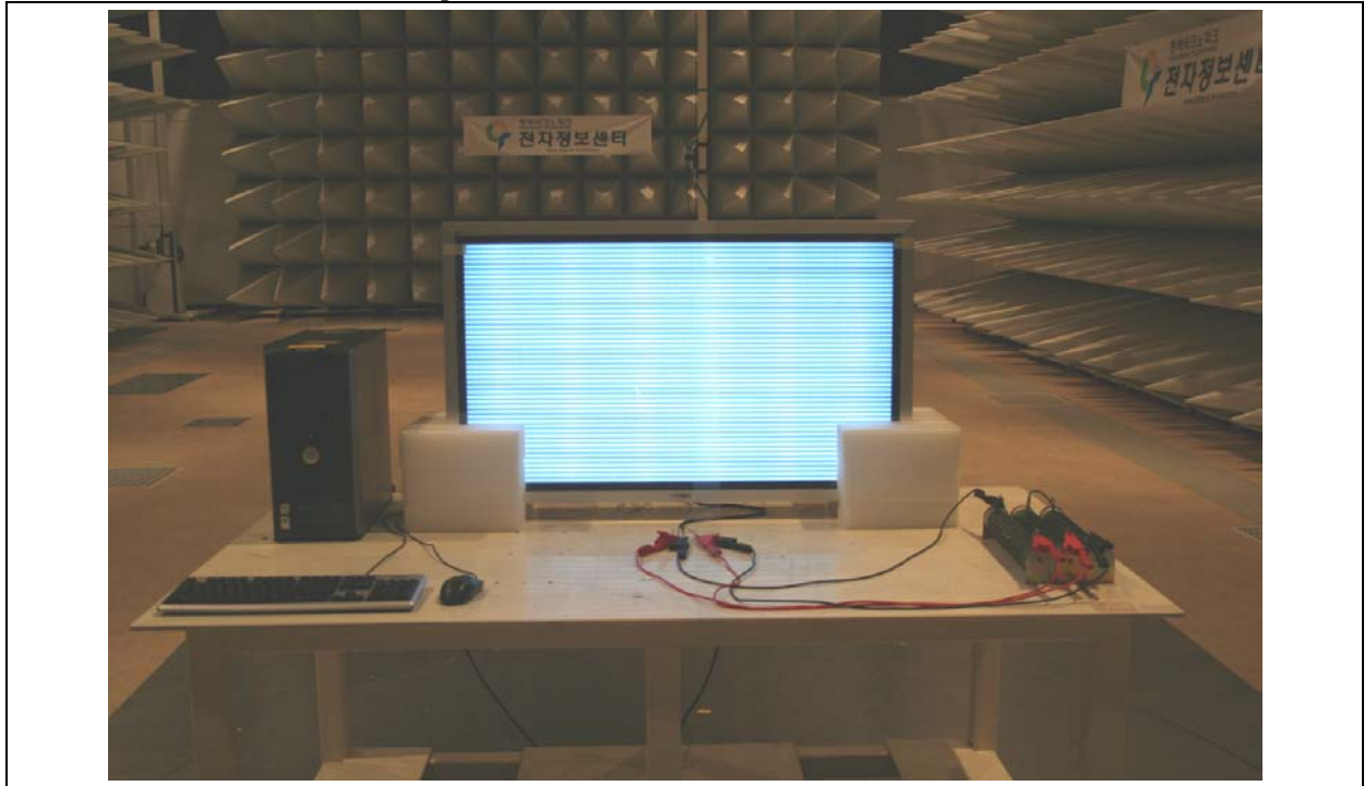
Figure 2 Photo of Radiated emission test setup: VGA and DVI Mode
