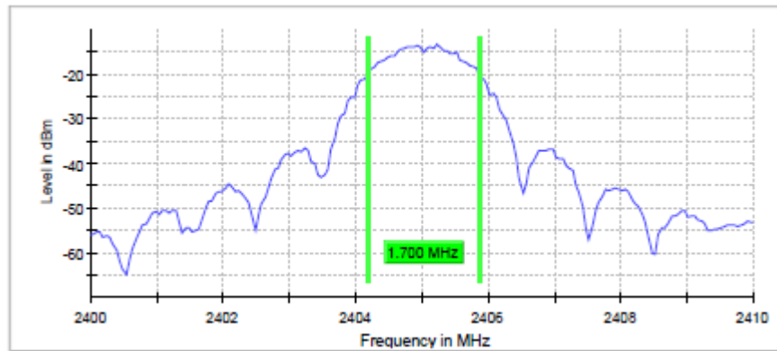
6 dB Bandwidth Plot on Configuration : Lowest channel (2 405 MHz)
