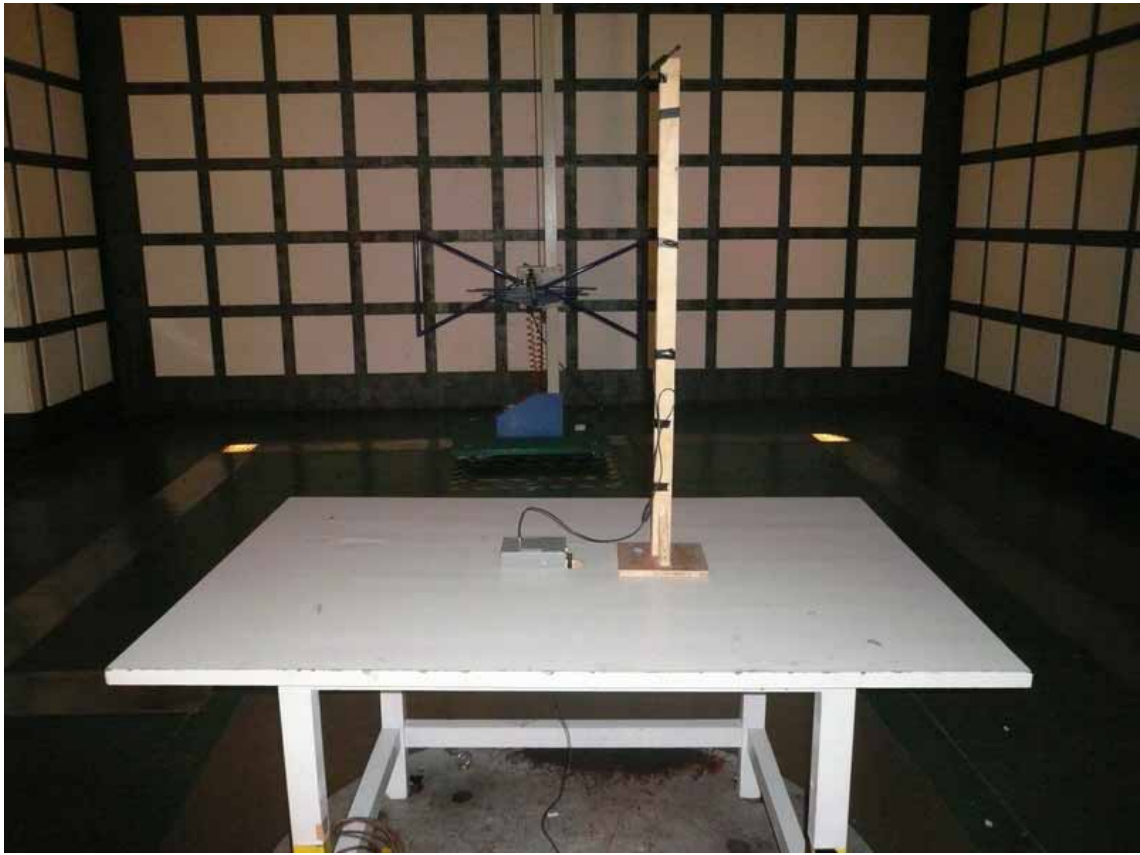
(Long antenna)
