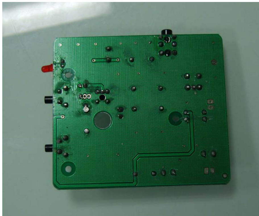
INTERNAL PHOTOS OF EUT – 2
