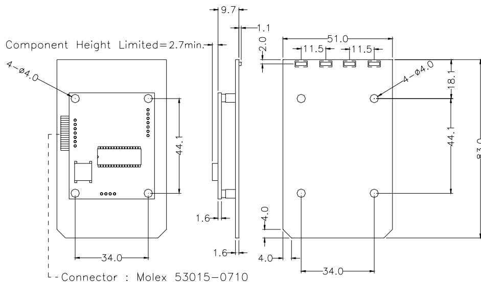
Figure 2-1 Dimensions of UIC680
