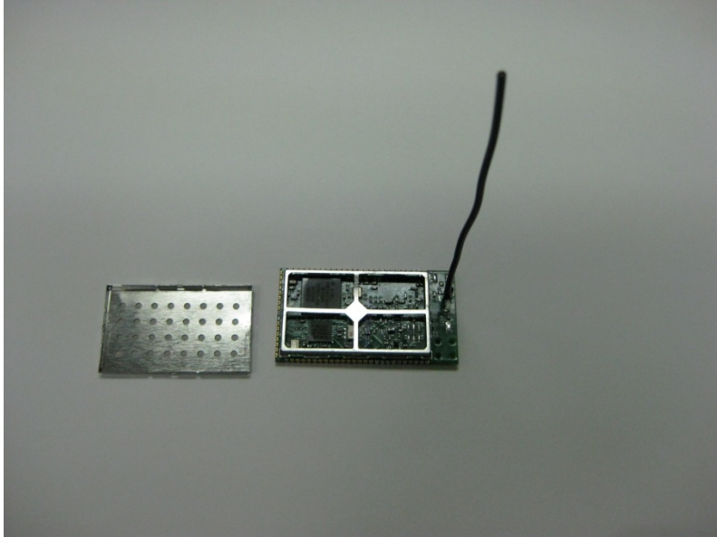
Photo of Unit with Wire Antenna
