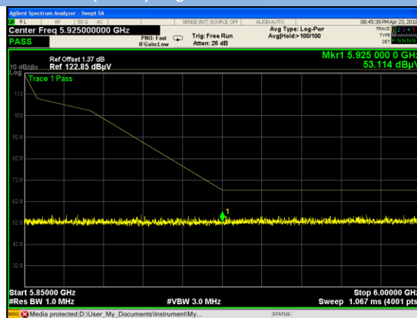
Band IV 11n(HT20) High channel, PEAK
