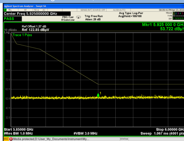
Band IV 11a High channel, PEAK
