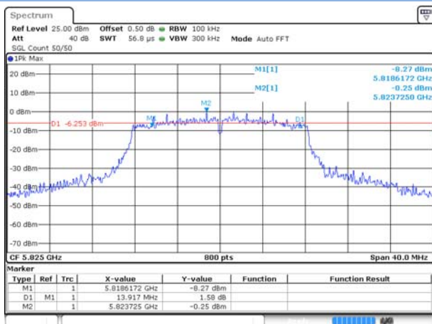
802.11a BAND IV HIGH CHANNEL
