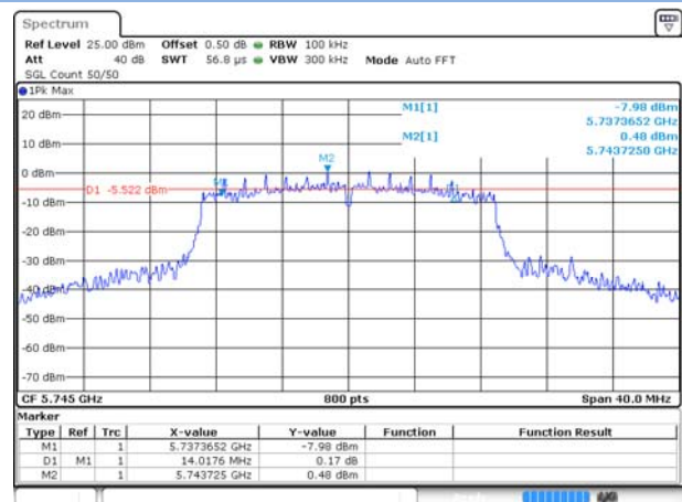
802.11n(20MHz) BAND IV LOW CHANNEL
