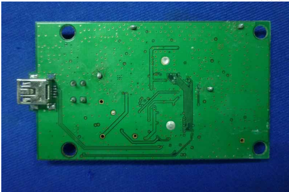
Figure 8 Inside of the EUT
