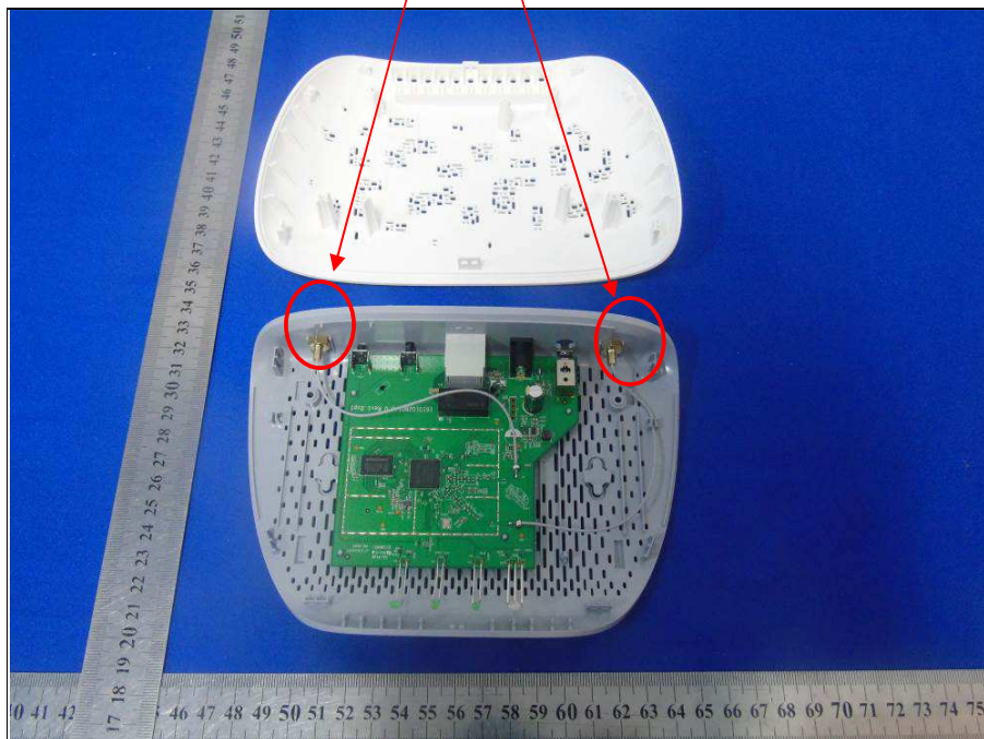
Antenna Connector
