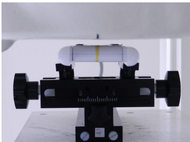
Back, Test Separation 0.5 cm Angle 180 Degree
