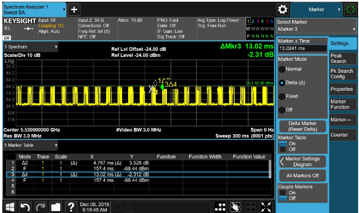
Channel Loading Plot - 802.11ac-VHT80 - 5530MHz
