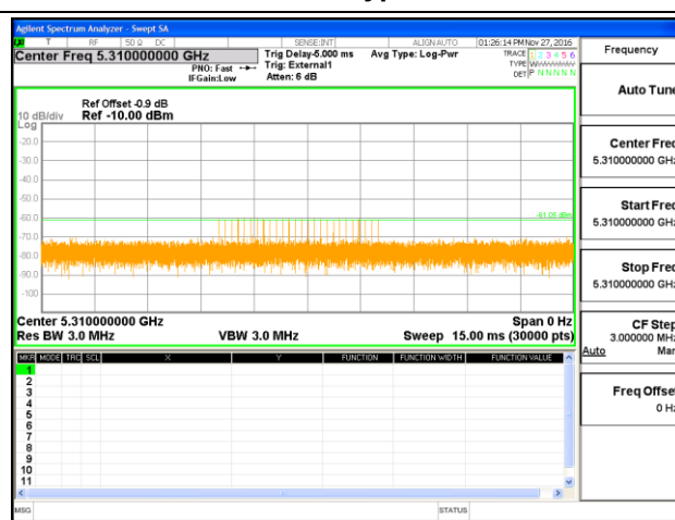
Radar Type 4
