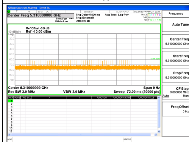
Radar Type 3
