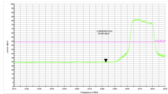
802.11g-Channel 1: Average
