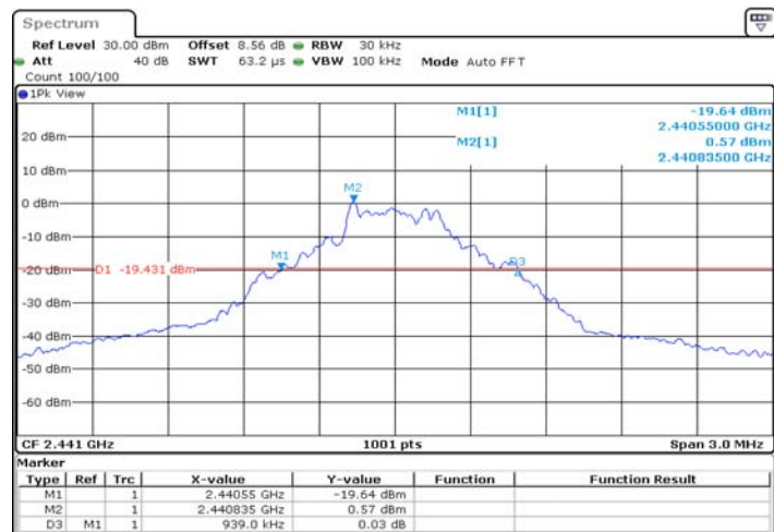
DH1_Ant1_2441
