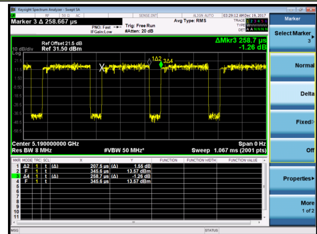
802.11ac-VHT40 (T = 207.5us)
