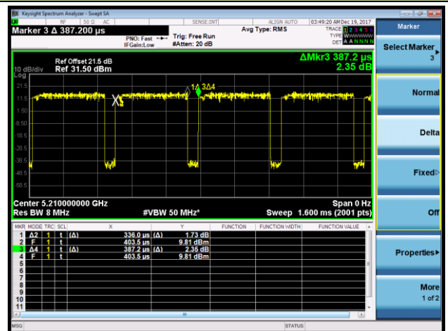
802.11ac-VHT80 (T = 336.0us)
