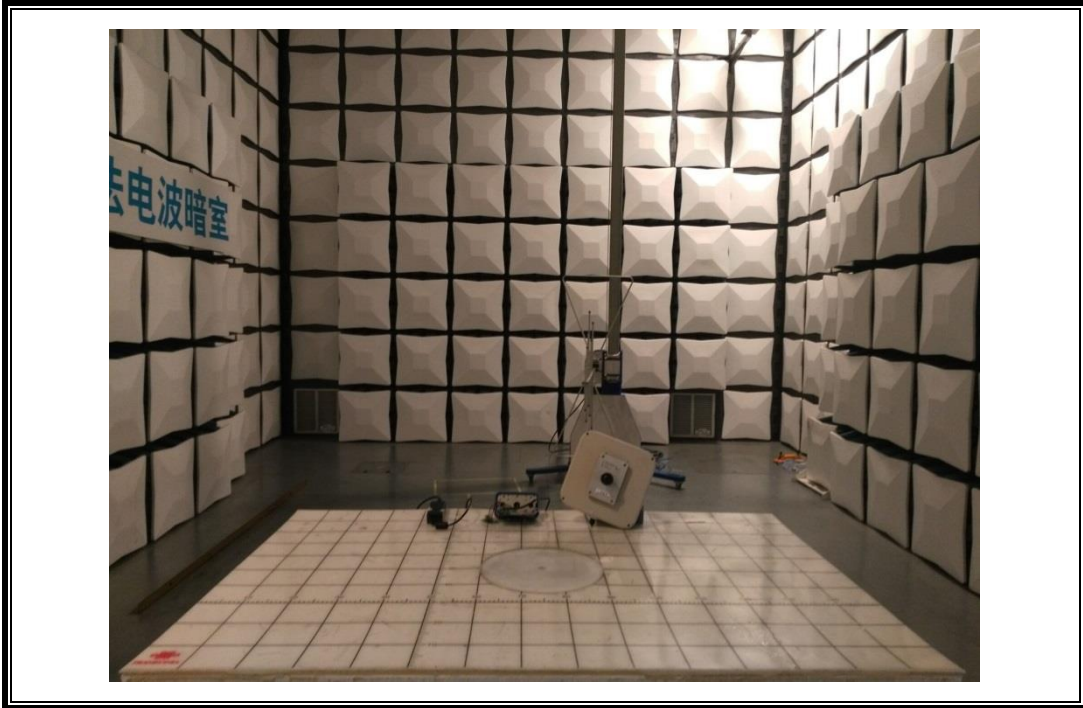
RADIATED RF MEASUREMENT SETUP (ABOVE 1 GHz)
