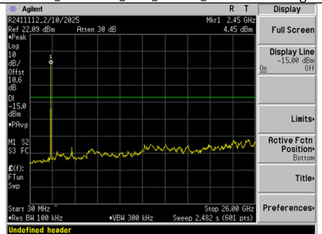
Mid Ch_2441MHz_3DH1_-20dBc_30-26GHz
