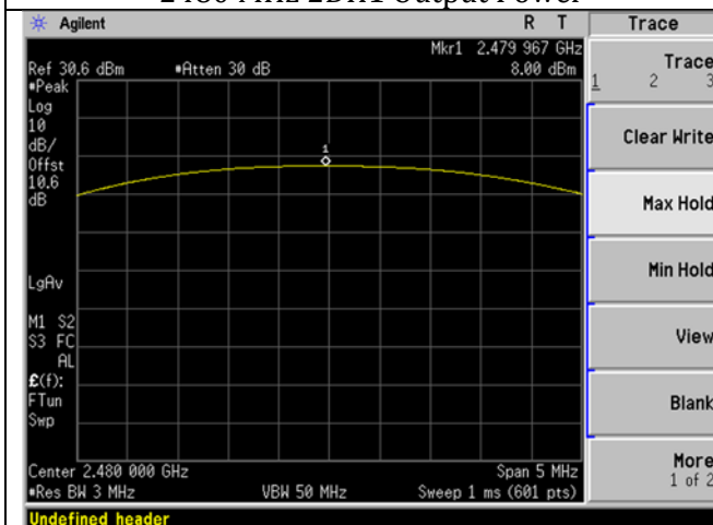
2480 MHz DH1 Output Power
