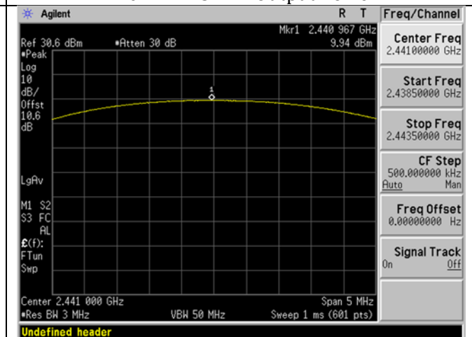
2441 MHz 2DH1 Output Power
