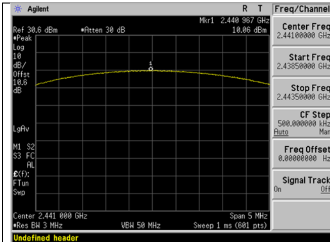
2441 MHz 3DH1 Output Power
