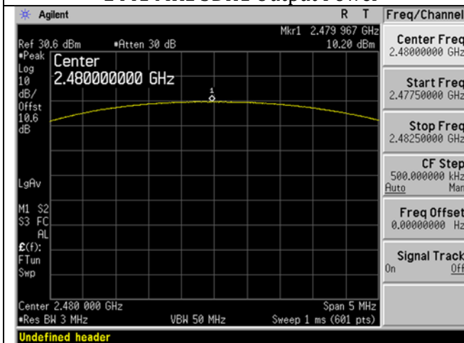
2480 MHz 2DH1 Output Power
