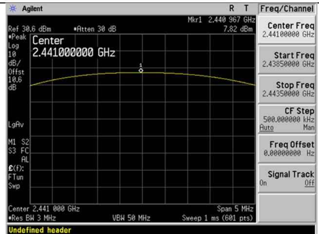
2441 MHz DH1 Output Power
