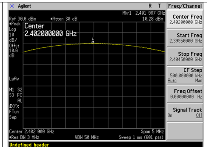
2402 MHz 3DH1 Output Power
